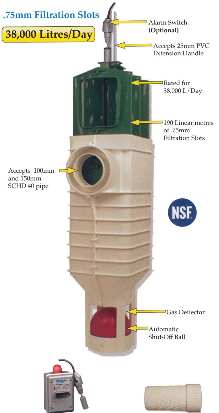
Outdoor SmartFilter® Alarm Polylok, Zabel & Best filters accept the SmartFilter® switch and alarm.
