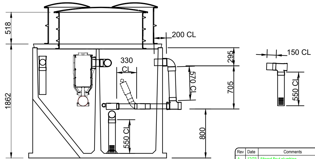
Section B-B
