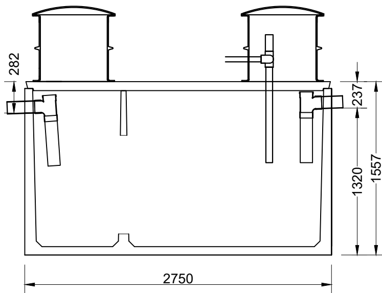
PTT13 same dimensions as ST33
