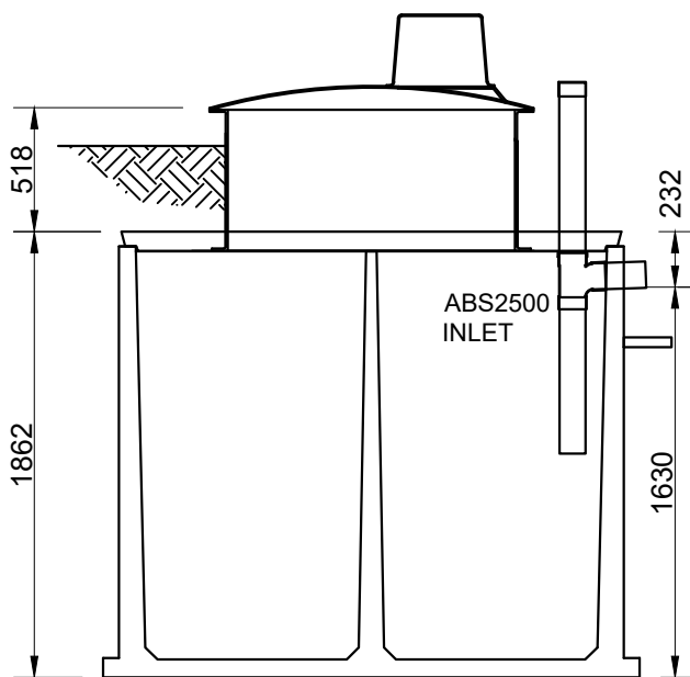
ABS2500 Dimensions as per ABS2000
